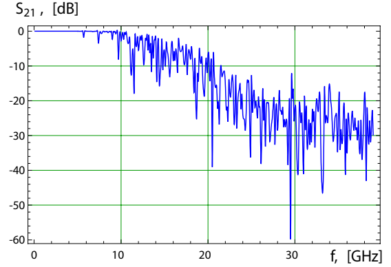
Figure 3: Transmission parameter S_{21} of the BPM insertion.
