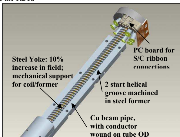
Figure 4: Details of the design of an undulator module. Undulator development has been underway in Europe by the HeLiCal collaboration [11]. A double helical coil, wound on a 6.35 mm diameter Cu tube, with an inner diameter of 5.85 mm, provides a helical transverse field. Successful tests of several prototypes have resulted in the choice for the RDR design [12]. A complete undulator
