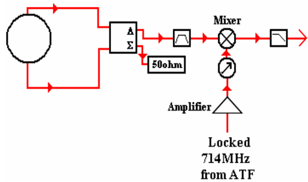
Figure 3: Schematic of FONT4 BPM signal processor.
