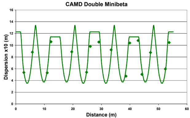
Figure 4: The calculated dispersion function x10 compared with the measured values.
