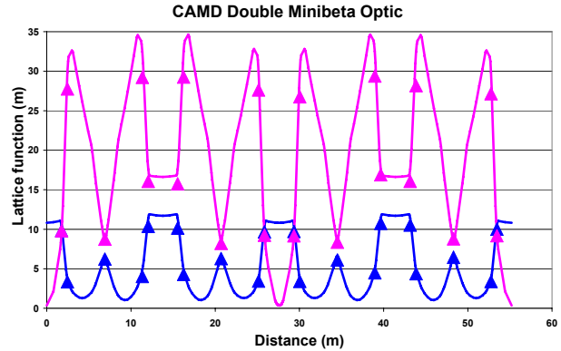
Figure 3: The calculated beta functions compared with the measured values averaged over each quadrupole. The vertical beta is shown red, the horizontal beta is blue.
