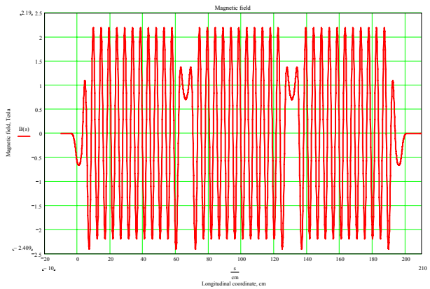
Figure 5: Magnetic field in the Multipole wiggler with the bump correctors energized.
