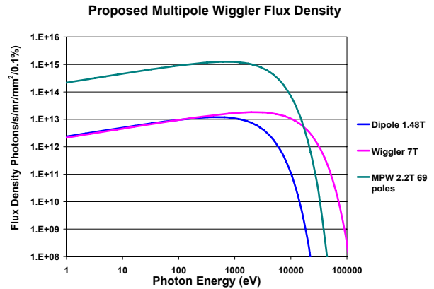
Figure 6: The flux density from the proposed multipole wiggler, the 7 Tesla wavelength shifter and the CAMD dipoles for a beam current of 250 mA.
