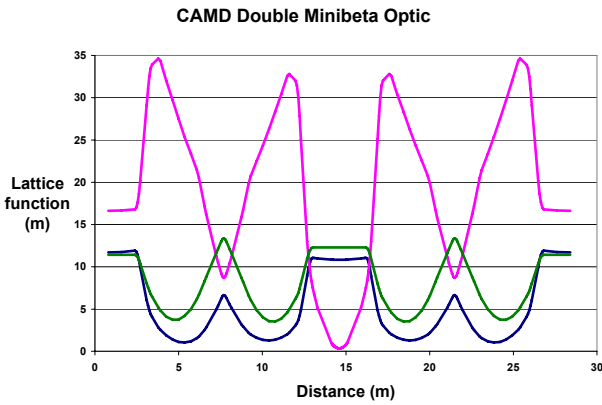
Figure 2: Double mini beta optic for CAMD. Half the circumference is shown. The vertical beta is shown red, the horizontal beta is blue and the dispersion x10 is green.
