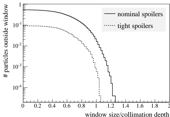
Figure 3. ‘Optimised’ ILC BDS collimation performance. For general description see Figure 1.
