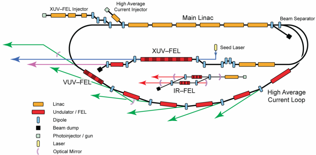
Figure 2. The conceptual layout of 4GLS.
