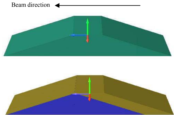
Fig. 1. Two different spoiler options. Top: Full titanium alloy body. Bottom: Graphite core covered by titanium alloy, which for the first taper the length of metal is of 0.6 \cdot X_0 . Visualized using SimpleGeo [7].
