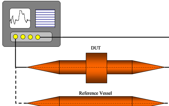
Figure 2: Schematic of the wire test apparatus.
