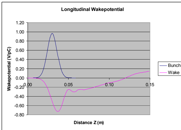
Figure 8: Longitudinal wakepotential for 6mm bunch.
