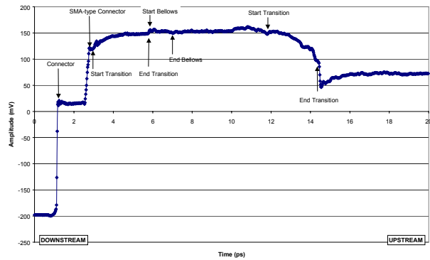
Figure 5: Example of the TDR Response.
