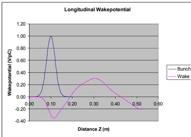
Figure 7: Longitudinal wakepotential for 20mm bunch.
