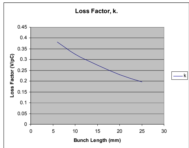
Figure 9: Loss factor versus bunch length.
